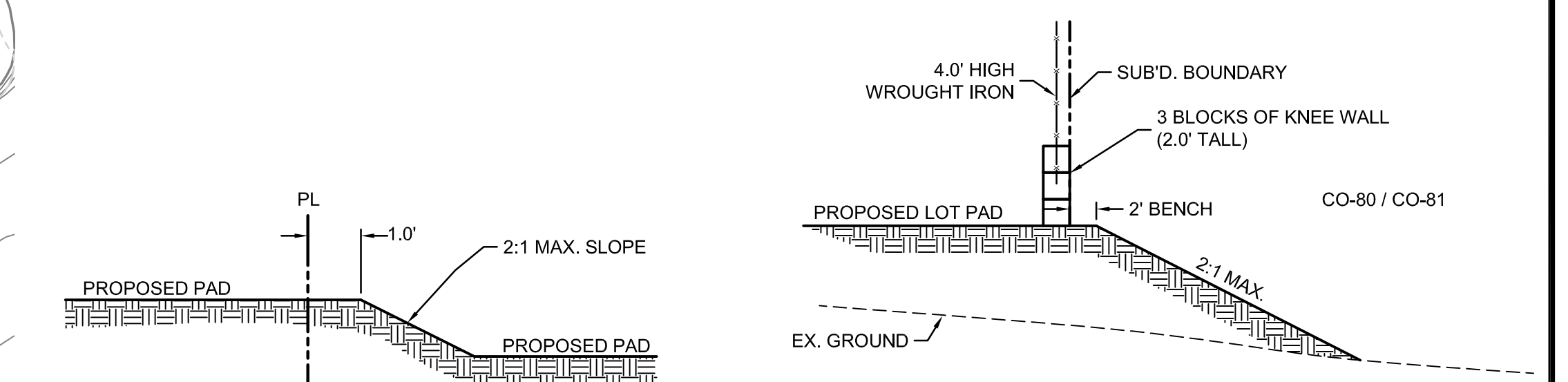
SECTION A-A TYPICAL SECTION WHERE THERE IS A STEP BETWEEN PADS NO SCALE
