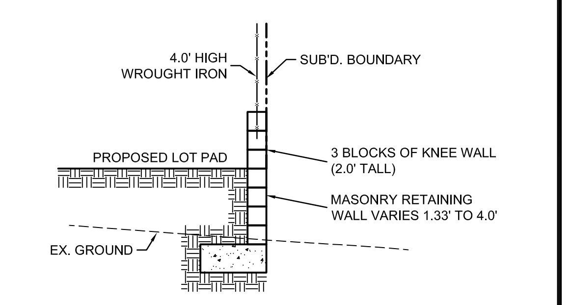
SECTION D-D NO SCALE
