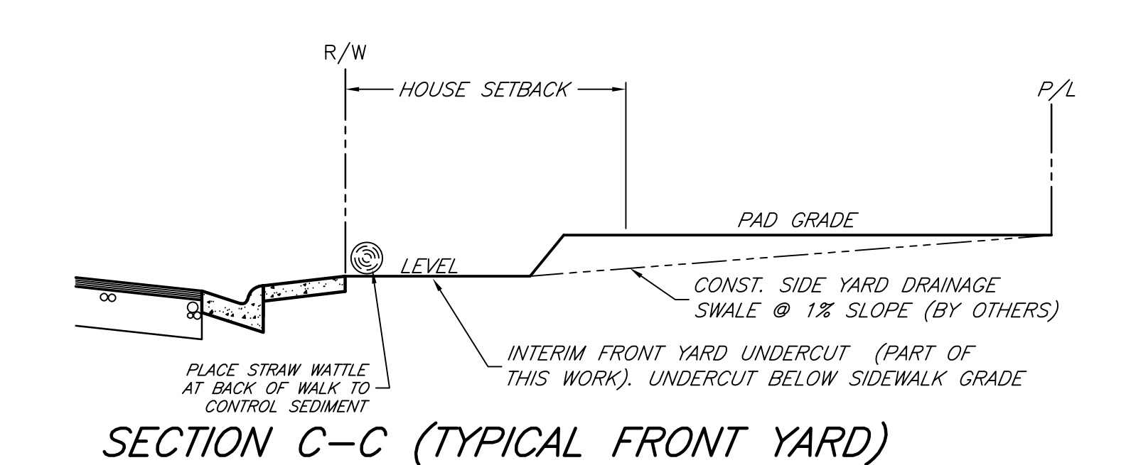
SECTION C-C (TYPICAL FRONT YARD) NO SCALE
