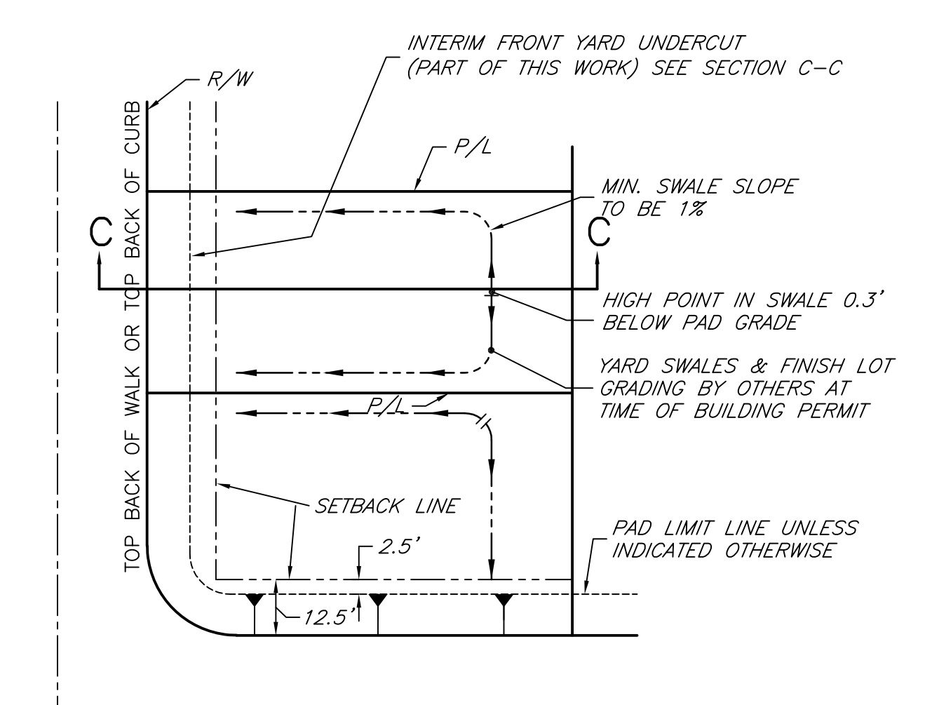
TYPICAL LOT GRADING NO SCALE
